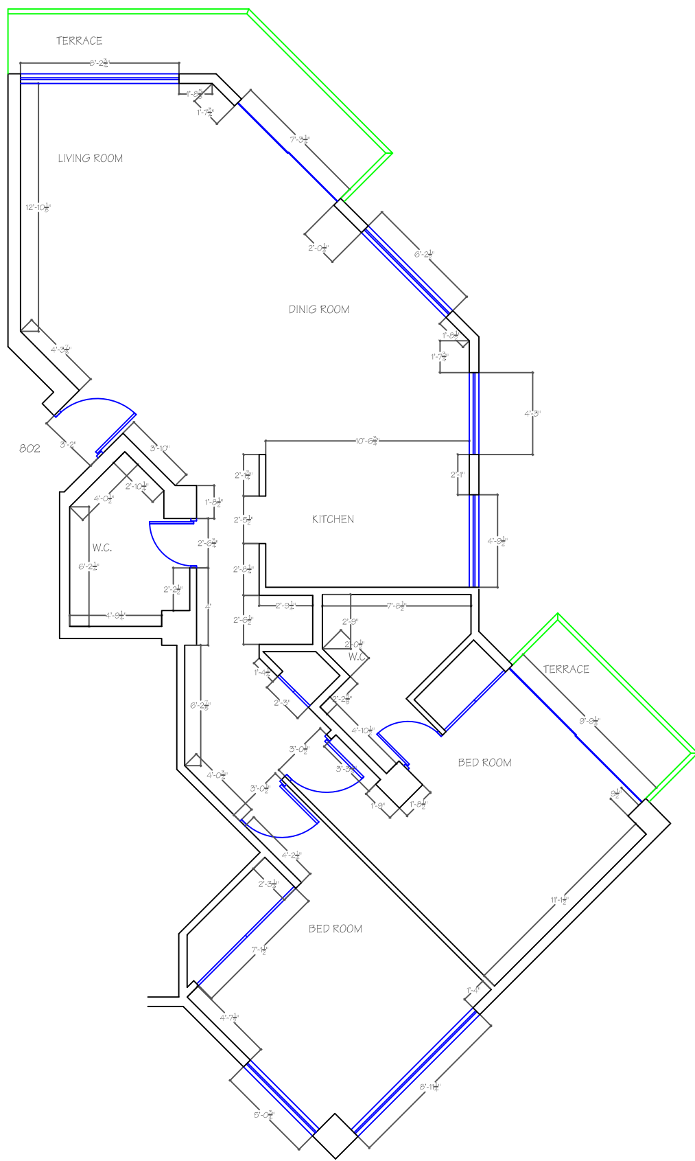
ARCHITECTONIC PLAN T-III 702 MEASURES
