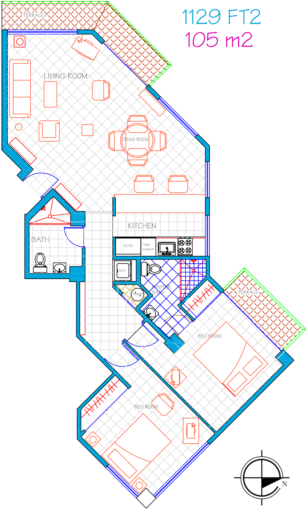
ARCHITECTONIC PLAN T-III 702 FURNITURE
