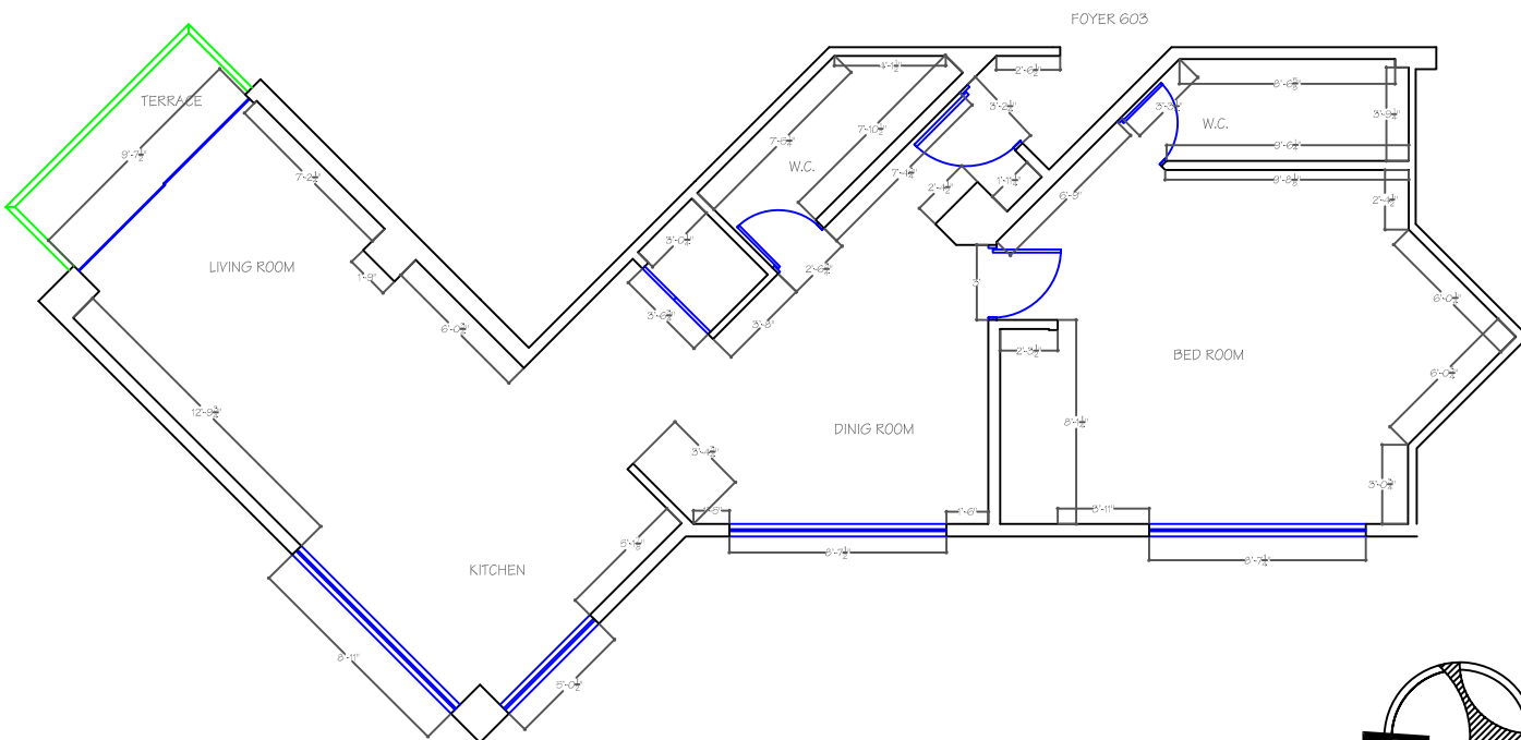
ARCHITECTONIC PLAN T-III 603 MEASURES
