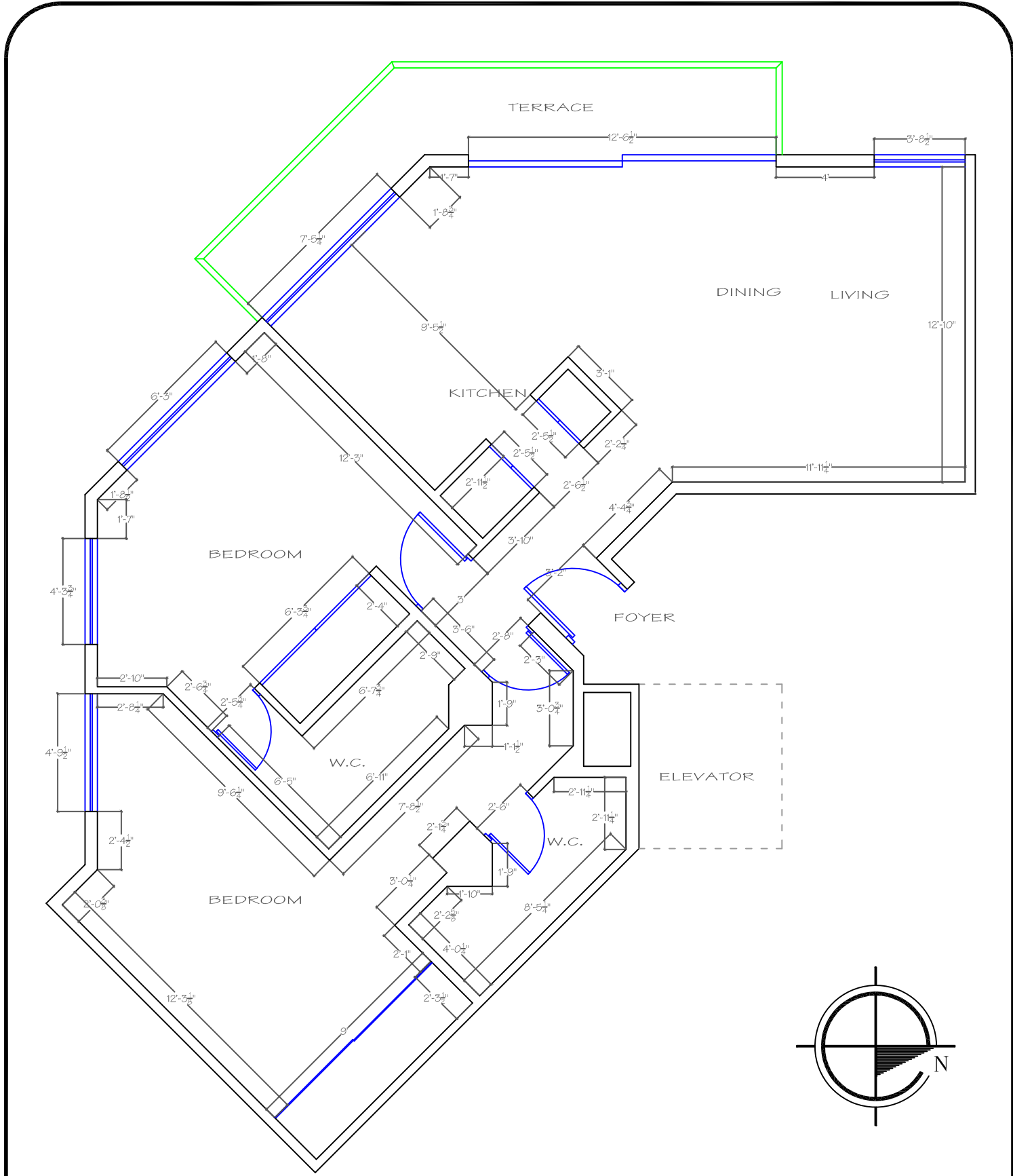
ARCHITECTURAL PLAN T-III 601 MEASUREMENTS
