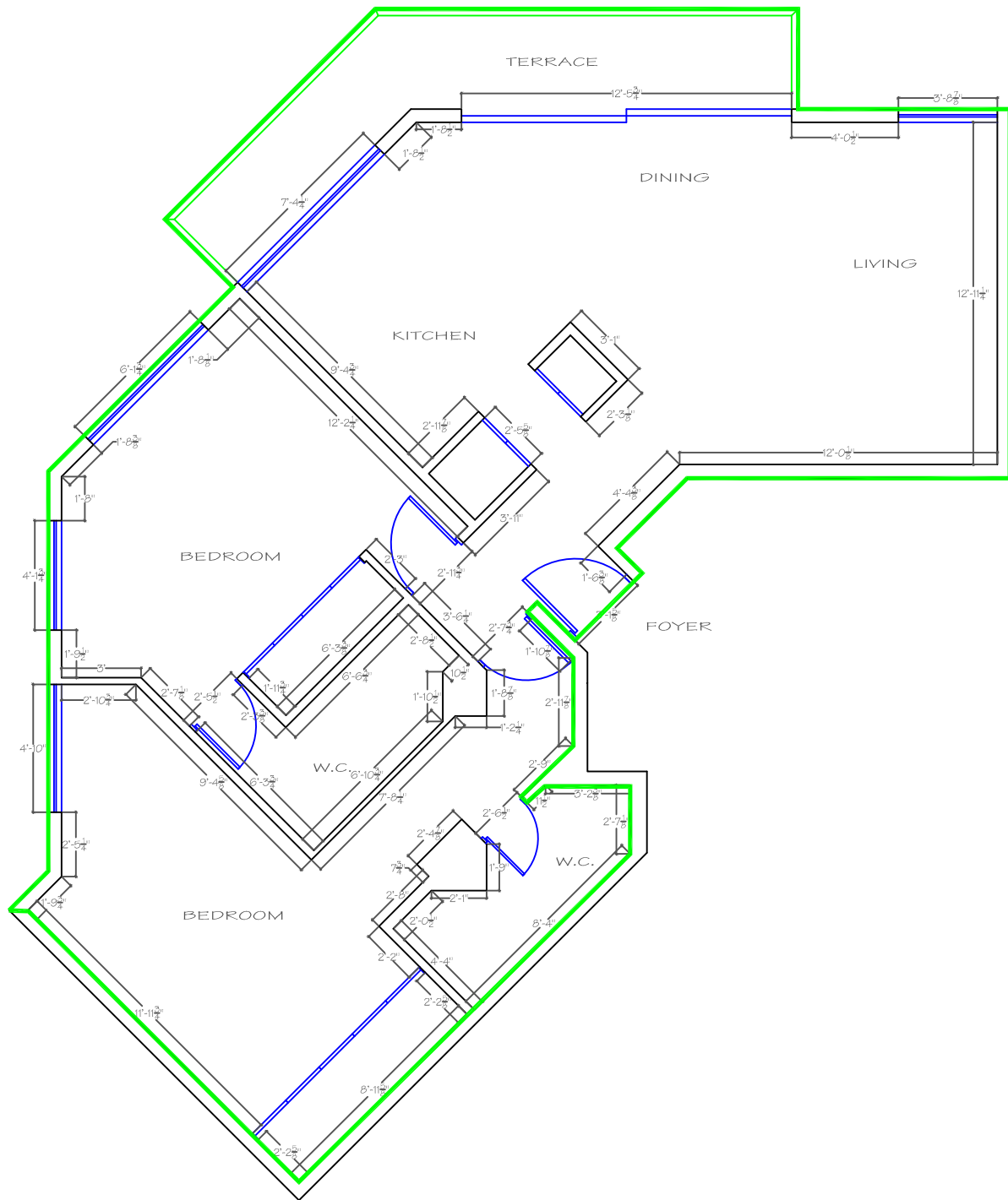
ARCHITECTURAL PLAN T-III 301 MEASUREMENT'S
