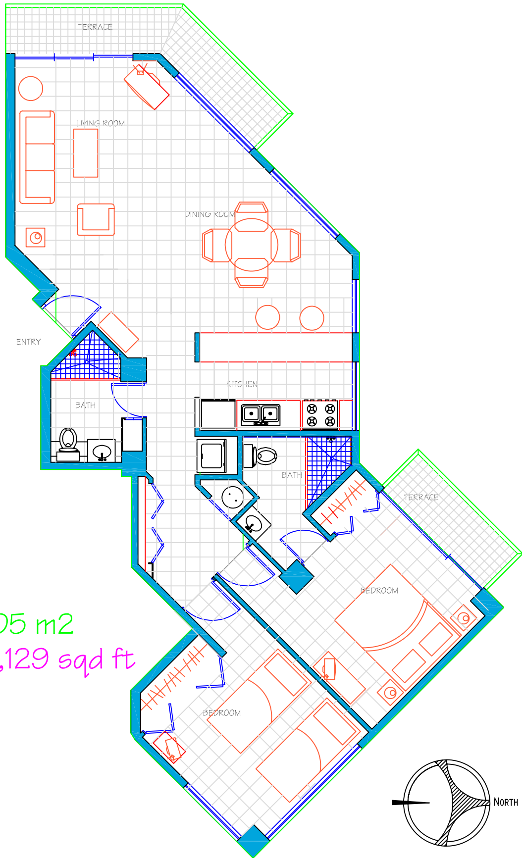
ARCHITECTONIC PLAN T-II 402 FURNITURE
