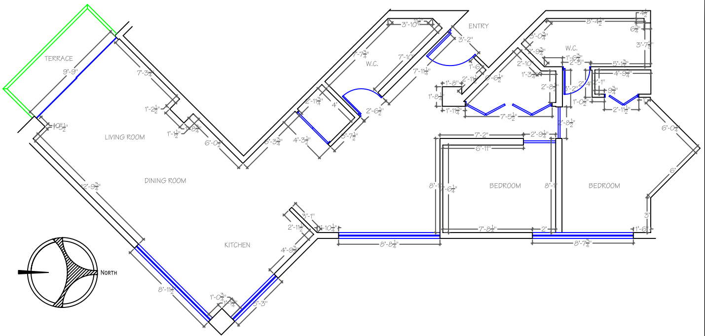
ARCHITECTONIC PLAN T-II 303 MEASURES
