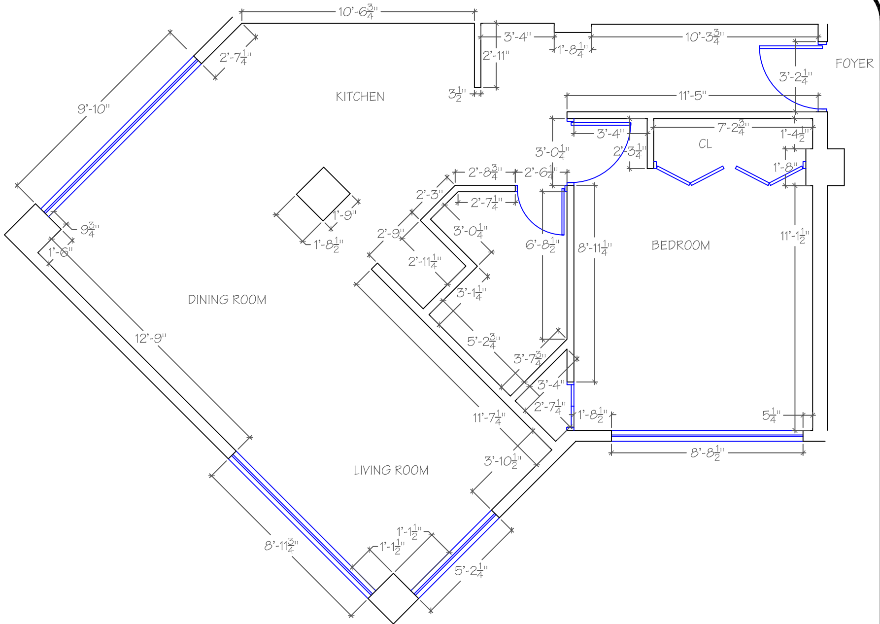
ARCHITECTONIC PLAN T-II 101 MEASURES
