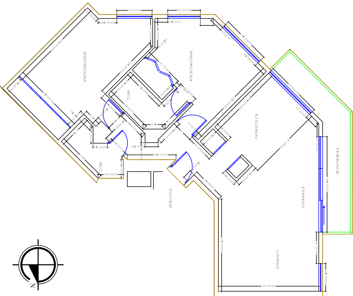
ARCHITECTONIC PLAN T-1 301 MEASUREMENT'S
