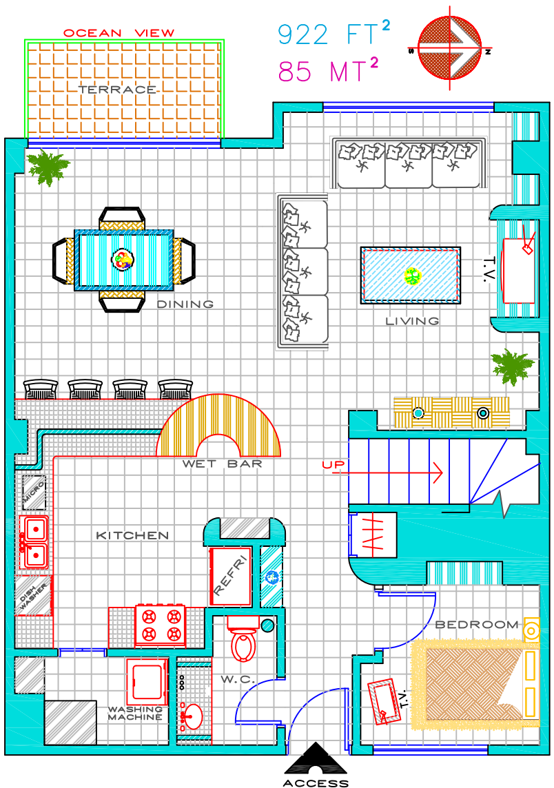
ARCHITECTURAL PLAN CM-902 FURNITURE'S
