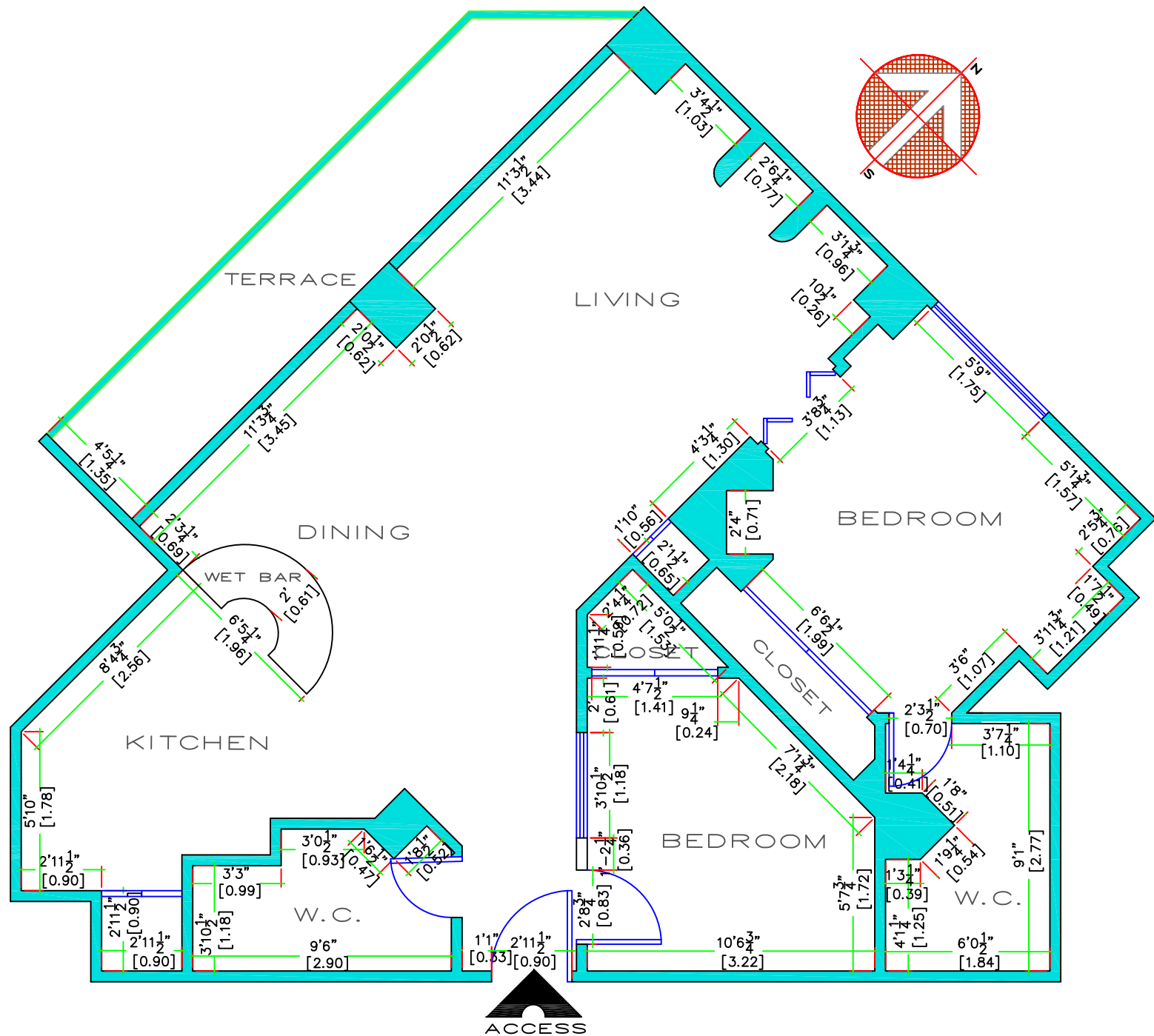
ARCHITECTURAL PLAN CM-510 MEASURES
