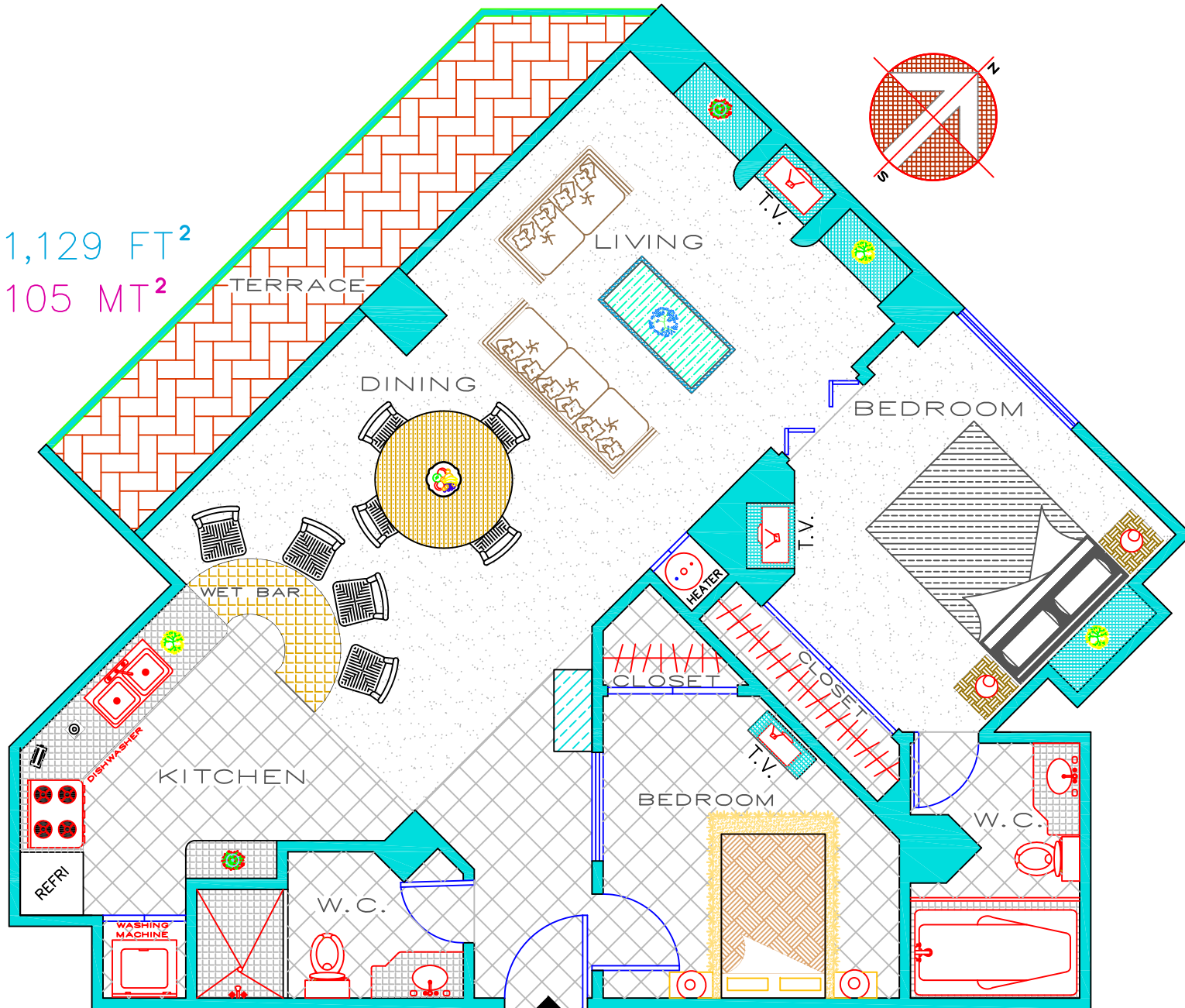
ARCHITECTURAL PLAN CM-510 FURNITURES
