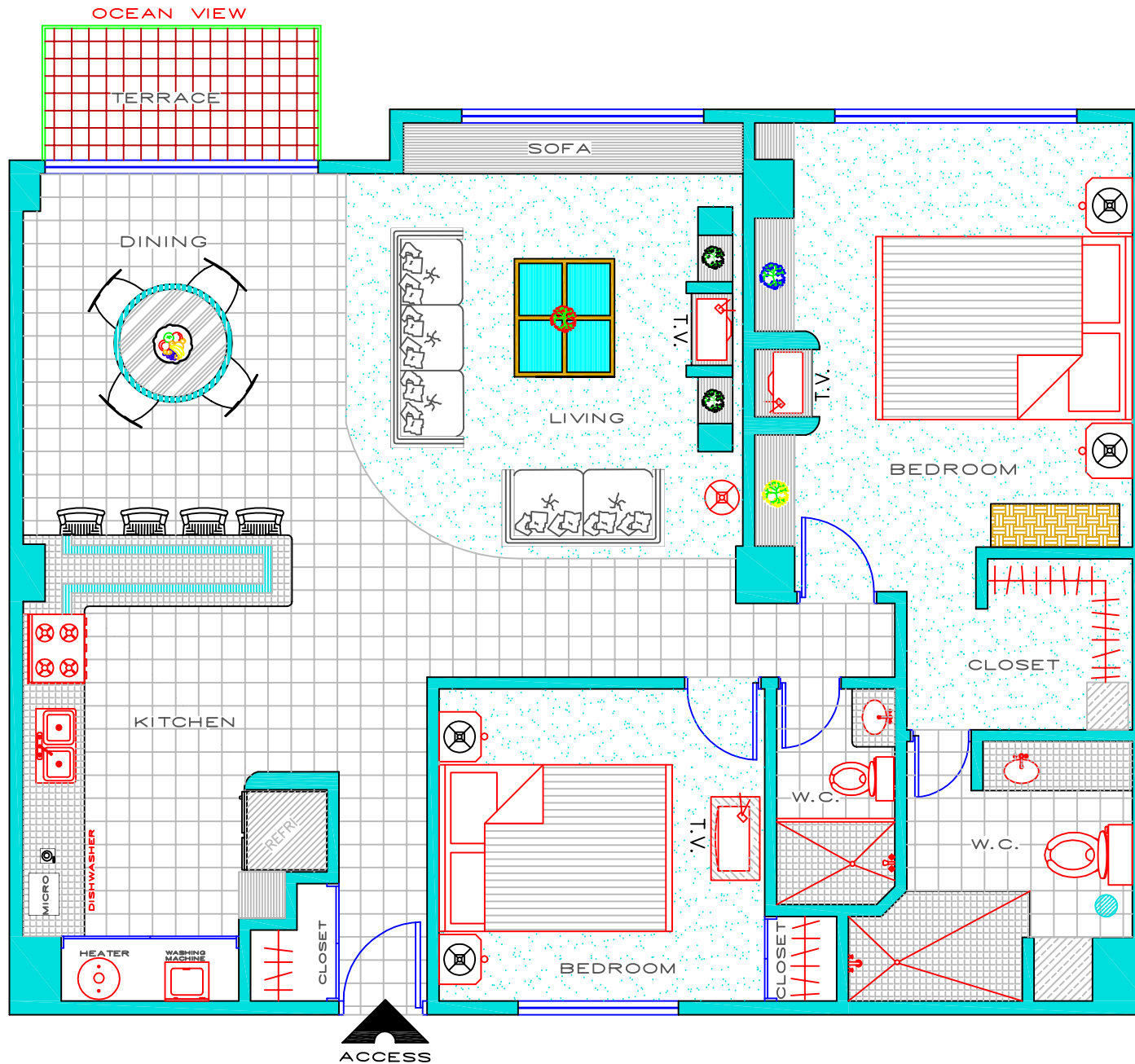
FLOOR PLAN
