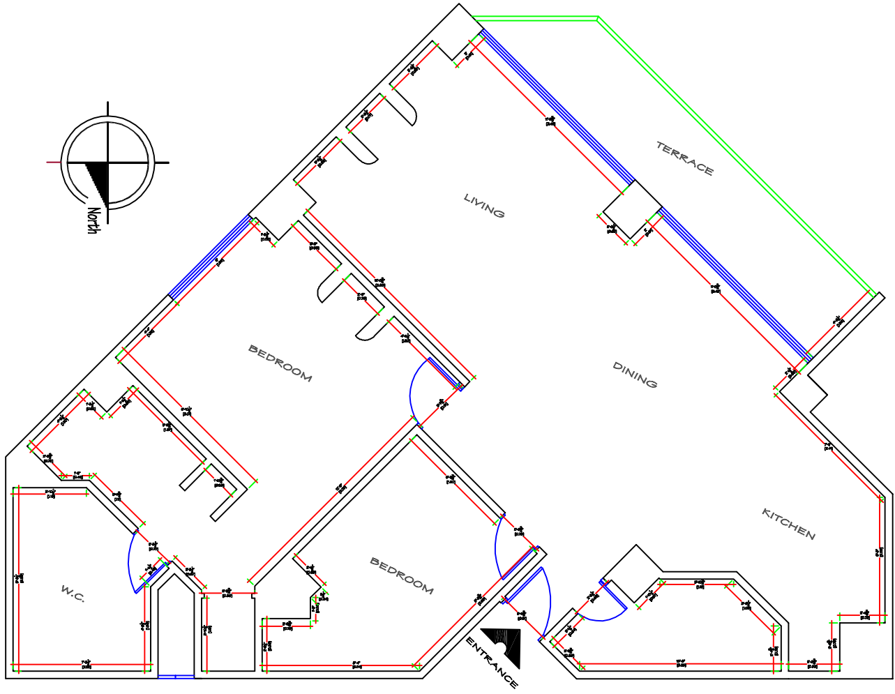
ARCHITECTURAL PLAN CM-407 MEASURES
