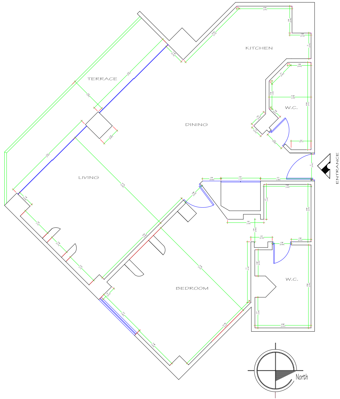
ARCHITECTURAL PLAN CM-309 MEASURES
