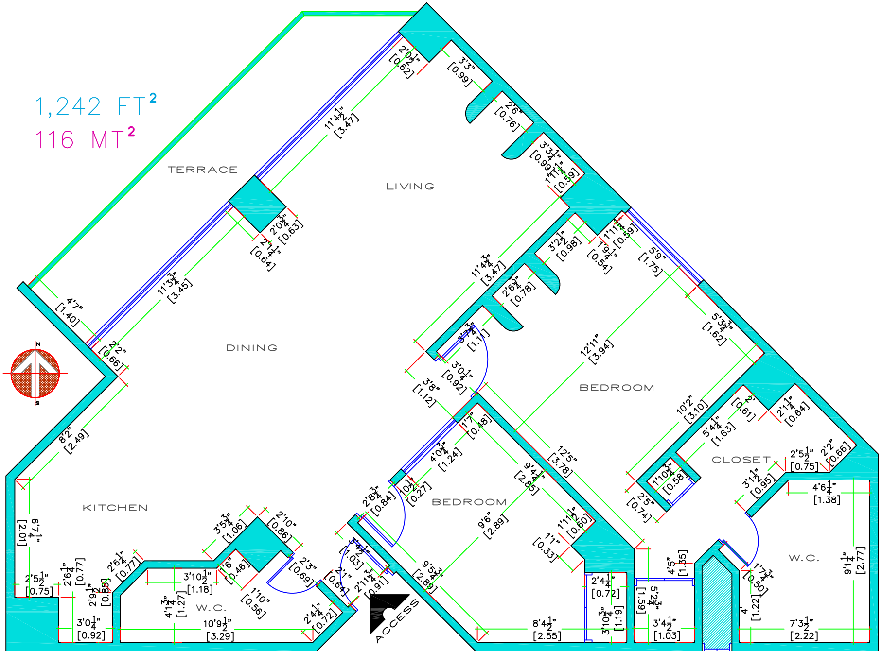
ARCHITECTURAL PLAN CM-308 MEASURE'S
