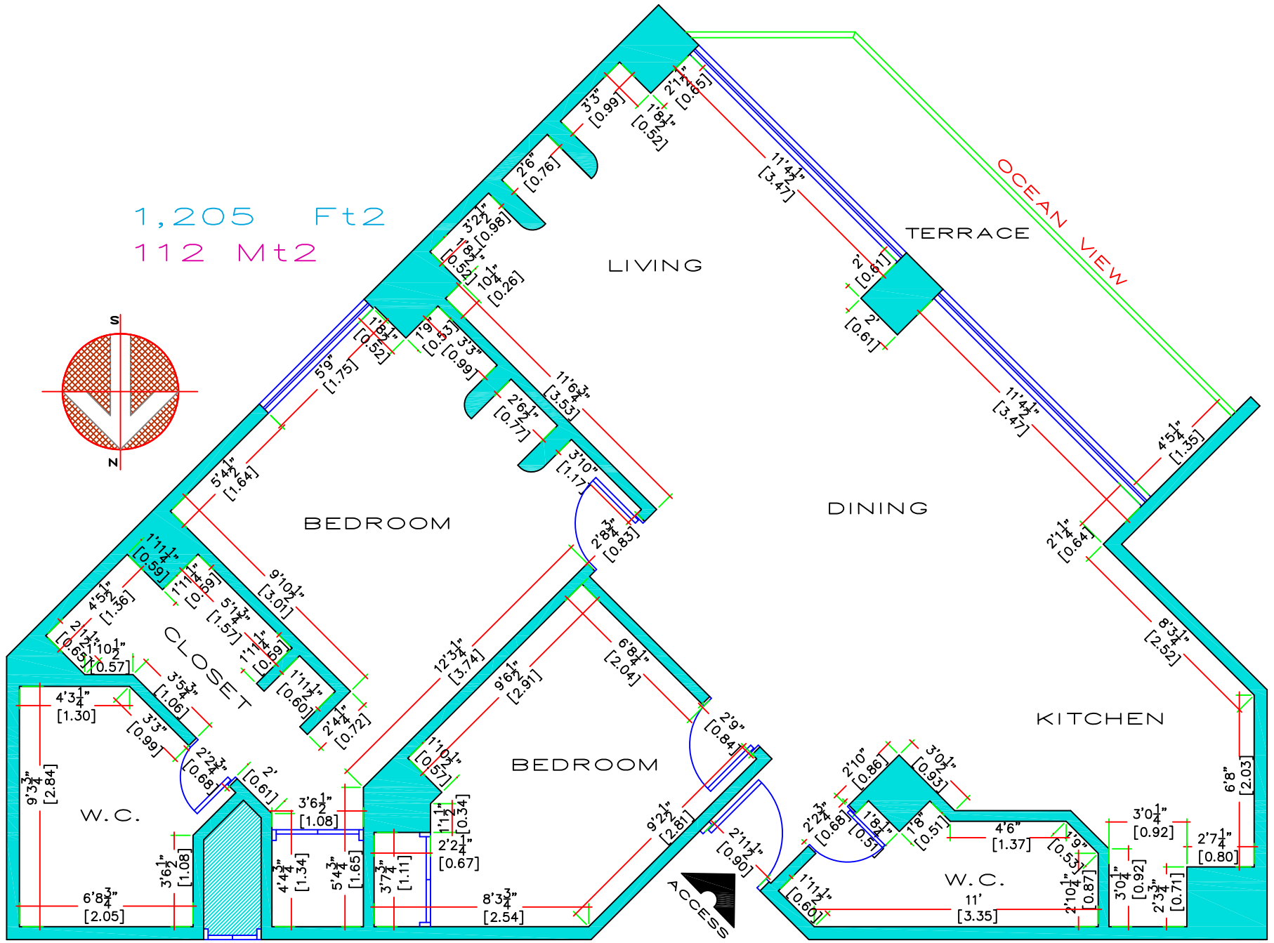
ARCHITECTURAL PLAN CM-307 MEASURE'S
