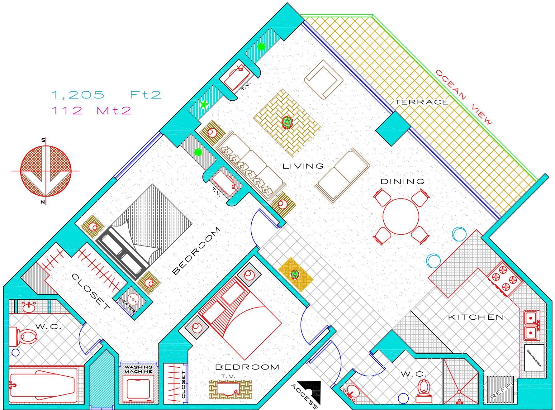
ARCHITECTURAL PLAN CM-307 FURNITURE'S
