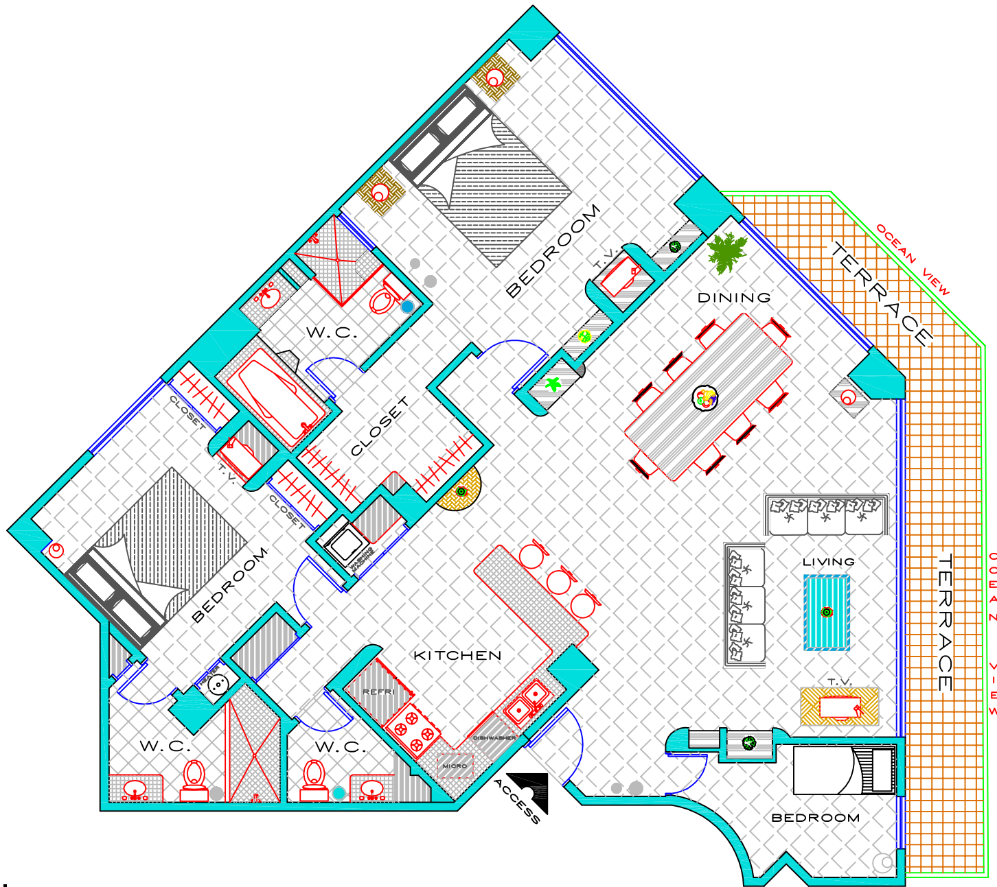
FLOOR PLAN
