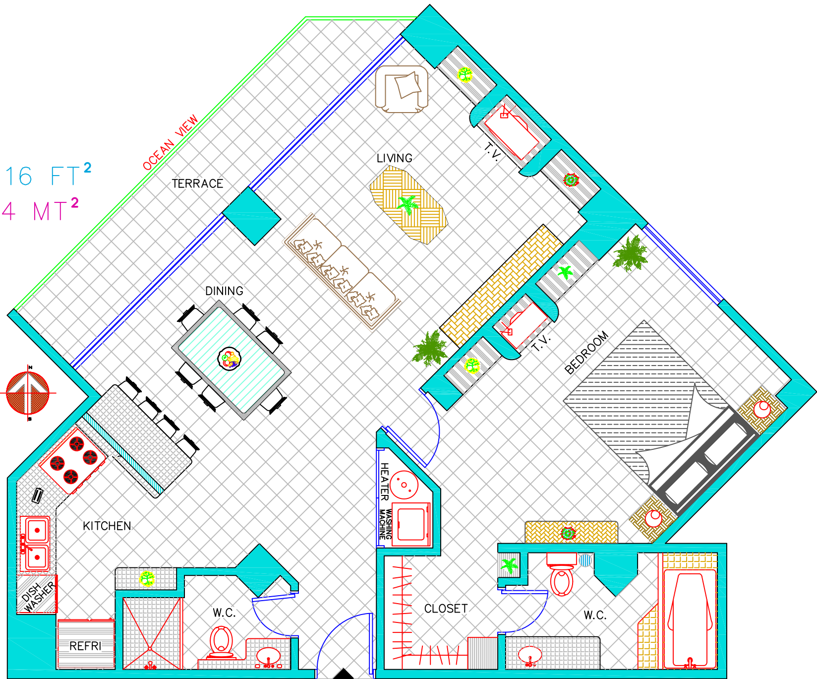
ARCHITECTURAL PLAN CM-1210 FURNITURE'S
