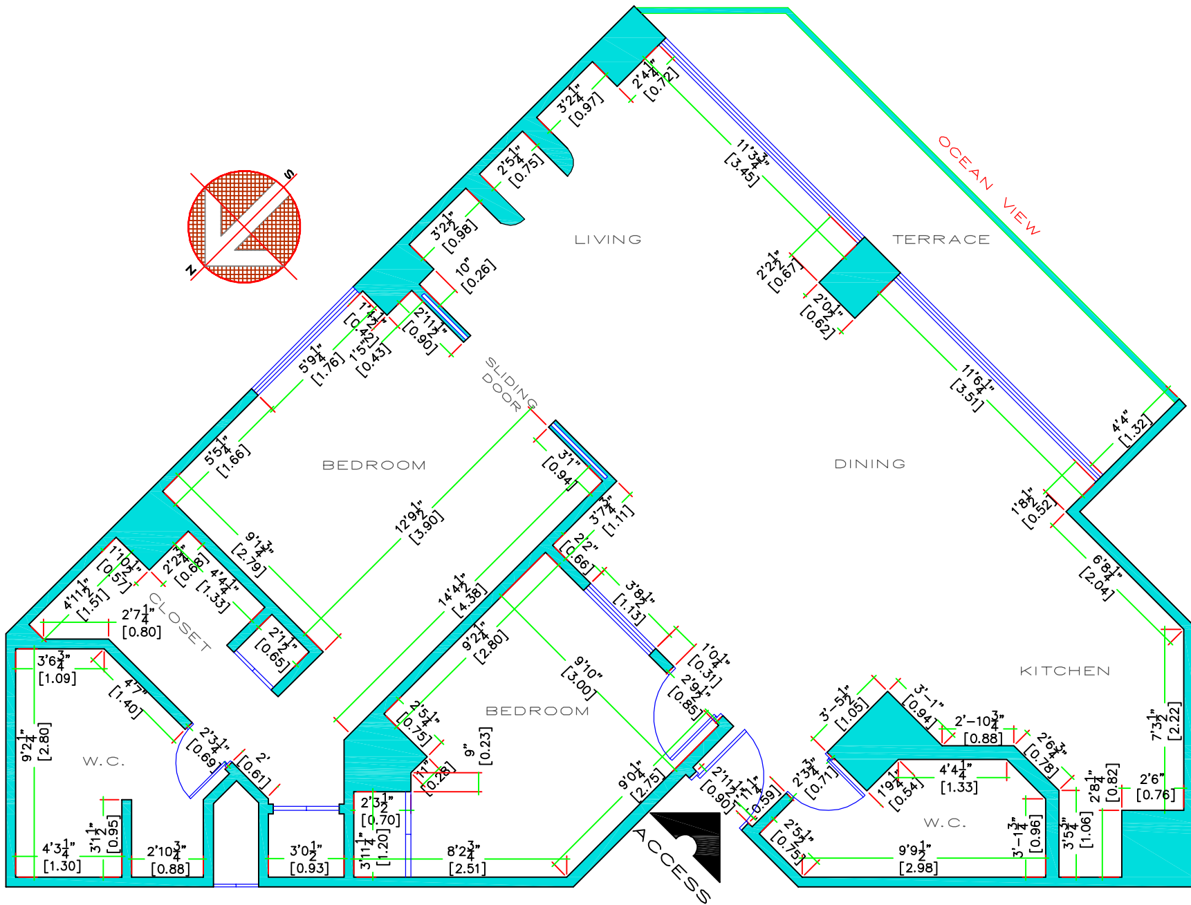
ARCHITECTURAL PLAN CM-1209 MEASURES
