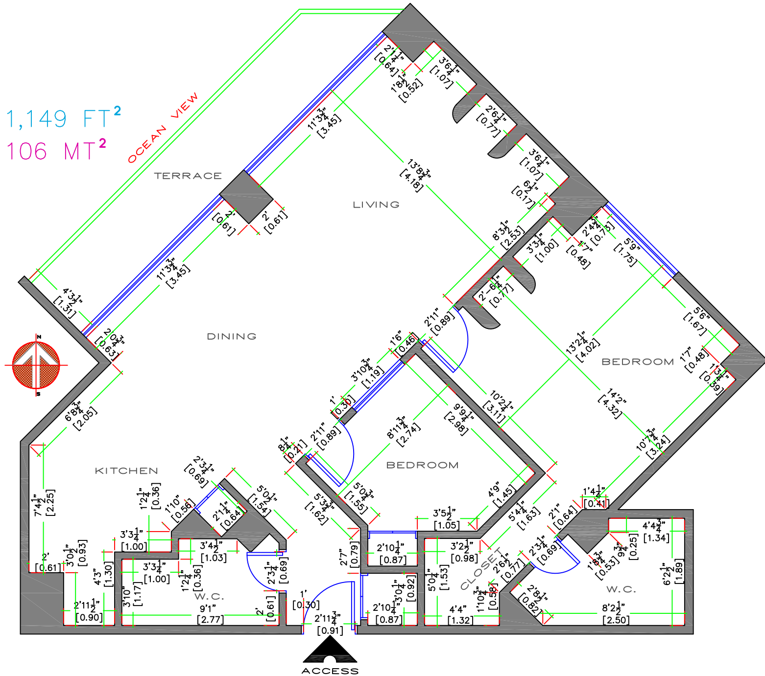
ARCHITECTURAL PLAN CM-III2 MEASURE'S
