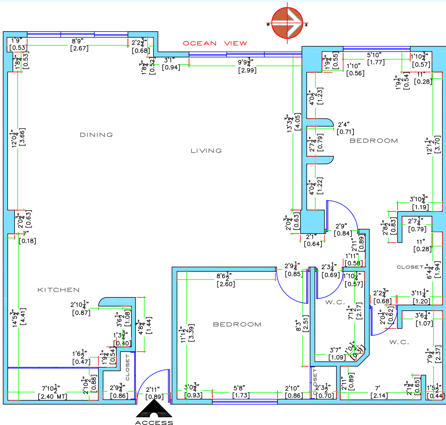
ARCHITECTURAL PLAN CM-104 MEASURE'S
